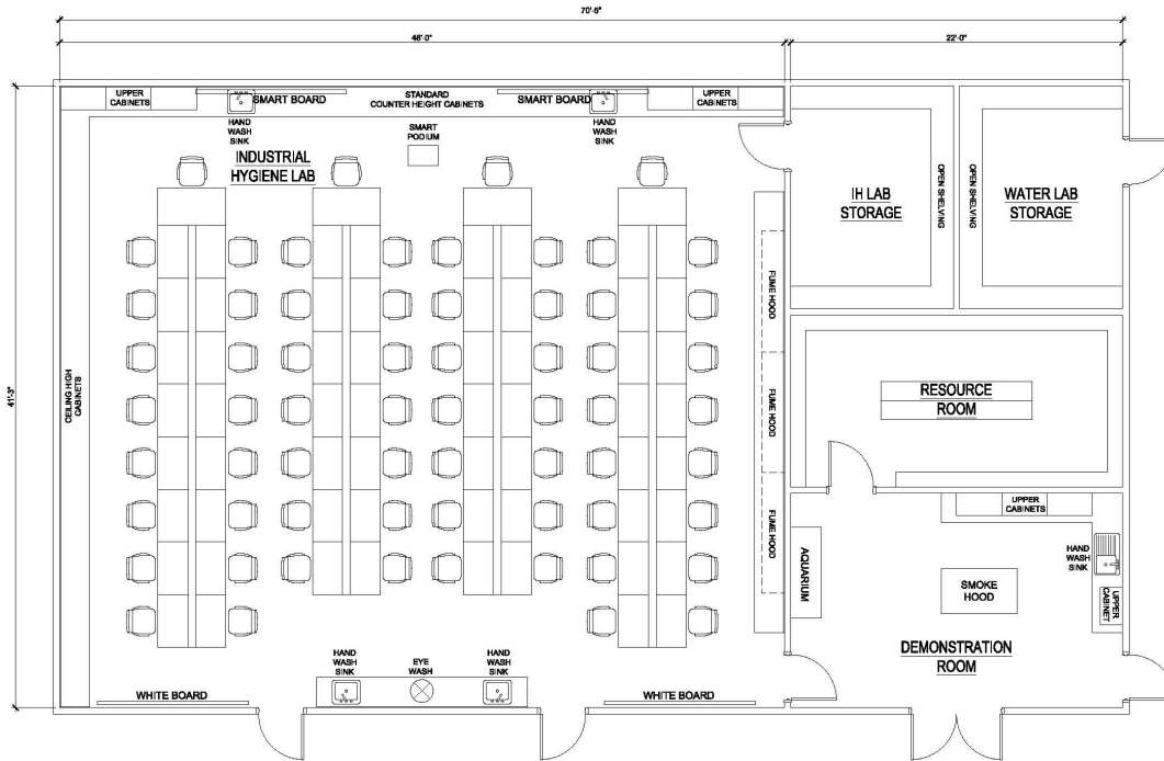
Figure 2. Planned preventive medicine industrial hygiene laboratory classroom (2,905 sq ft) for the consolidated and integrated enlisted preventive medicine instructional facility at Fort Sam Houston, Texas.
